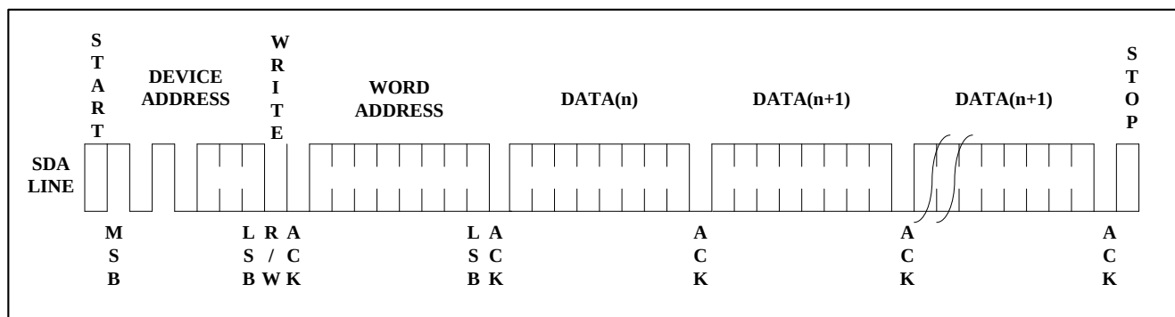
Figure 7. Page Write
