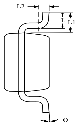
COMMON DIMENSIONS (UNITS OF MEASURE = MILLIMETER)
