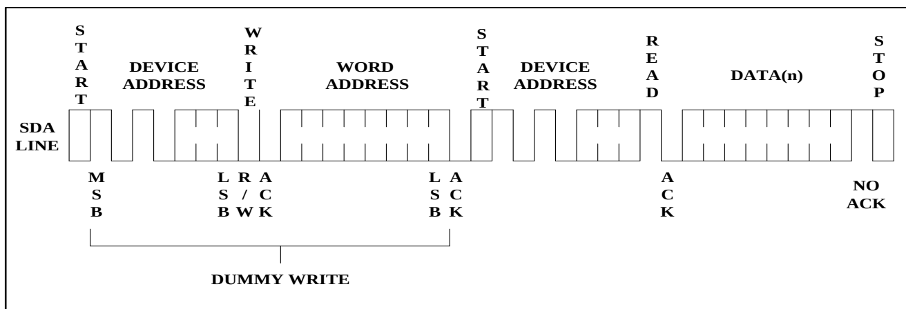
Figure 9. Random Read
