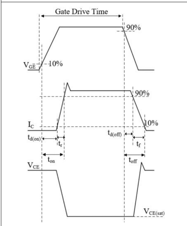
Figure 20 Switching Waveforms
