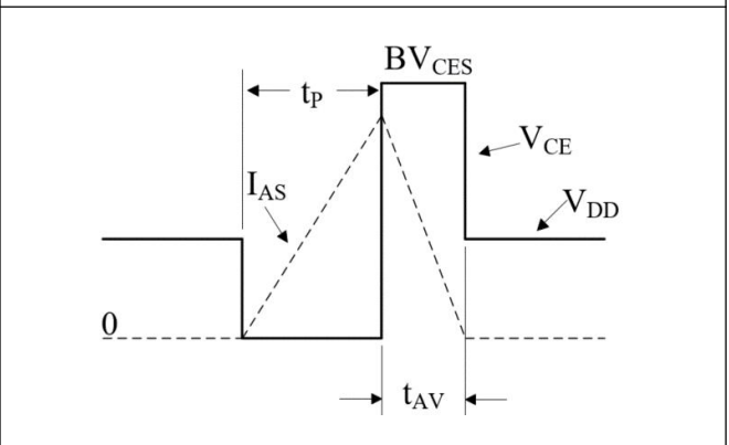
Figure 22 Self Clamped Inductive Switching Waveform
