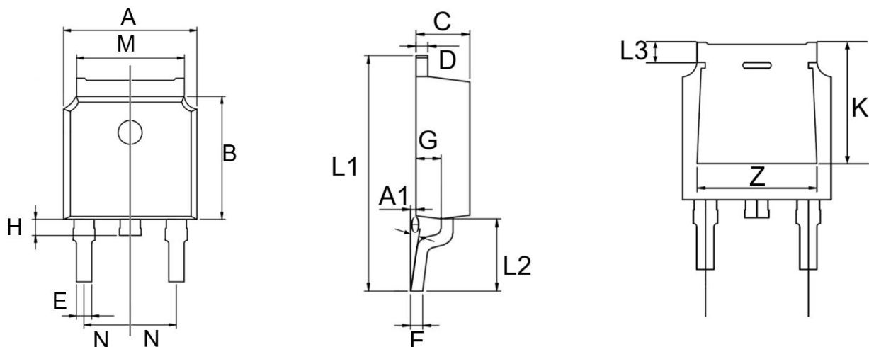
TO-252 Package
